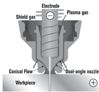
Conical Flow
